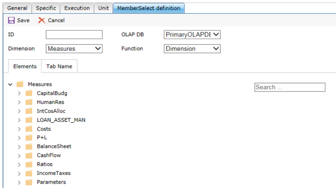
Fig. 31 - Member Select Designer
